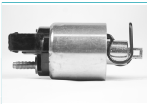
Solenoid Switch
