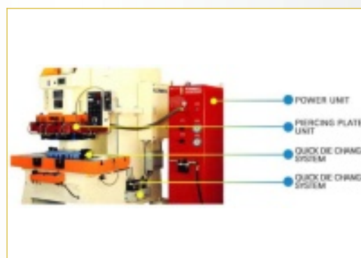
PCB Fine Piercing System
