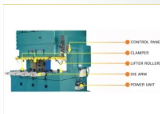
QUICK DIE CHANGE SYSTEM
