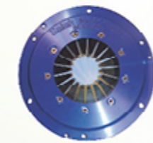
競技離合器及壓板 (多片式) Clutches and Clutch Pressure Plates for Racing Cars (Multi-Plate Type)
