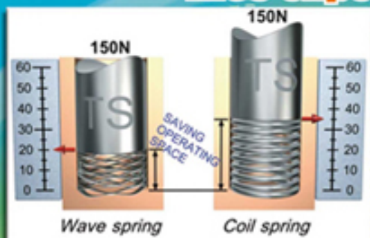
Wave Spring & Coil Spring
