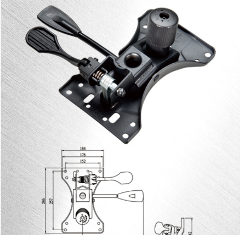
Seat Mechanism
