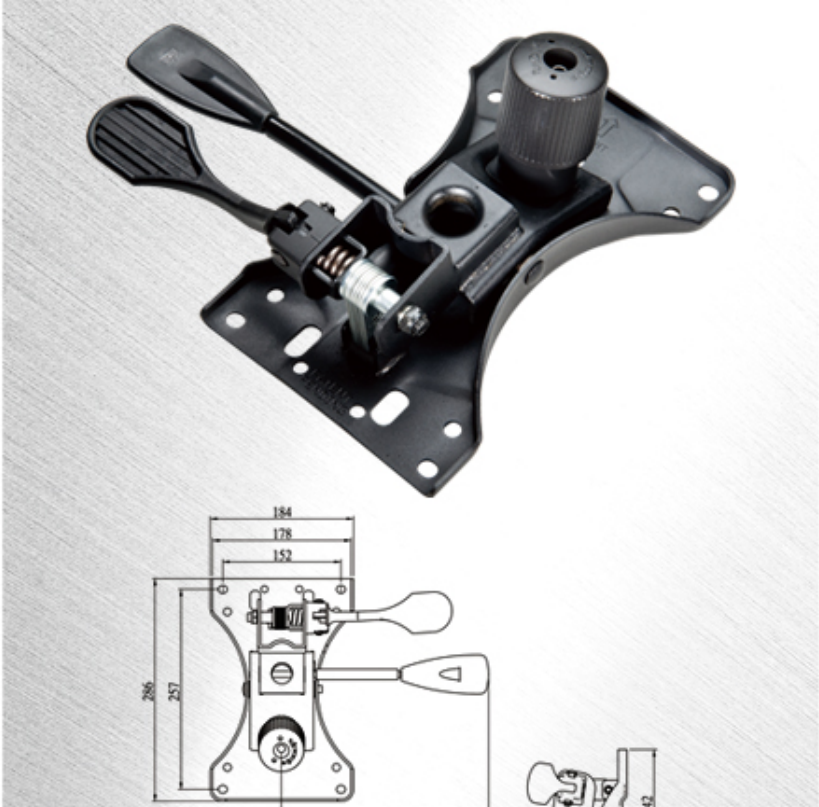
Seat Mechanism
