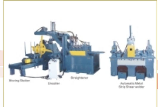
Metallic strip auto shear welder / Automatic Metal Strip Shear welder
