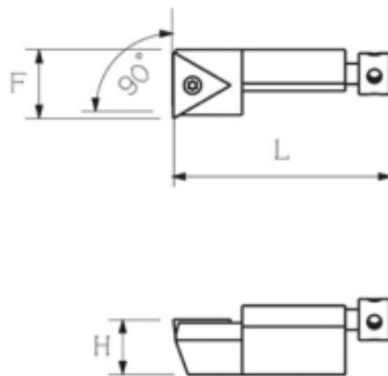
CNC Cartridge
