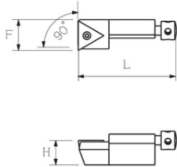
CNC Cartridge
