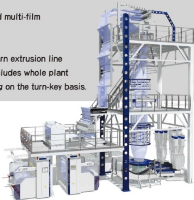
Multi-layer Co-extrusion Blown Film Extruder JC-CX Series
