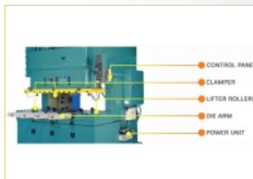
QUICK DIE CHANGE SYSTEM
