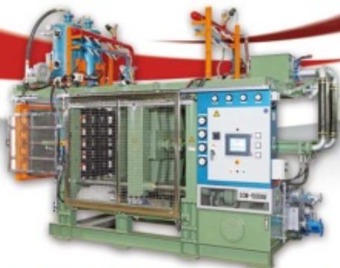
Fully automatic EPS/EPE shape-molding machine (AV-J series) 全自動EPS/EPE泡塑成型機 (AV-J系列)
