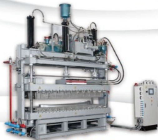
Automatic vertical EPS / EPE special-purpose molding machine 全自動立式EPS / EPE專用機
