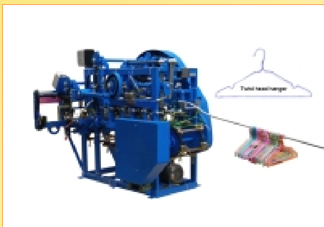
Automatic Clothes Hanger Forming & Making Machine
