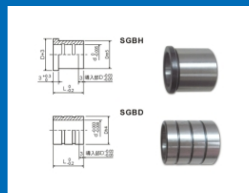
Guide Bush
