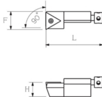
CNC Cartridge
