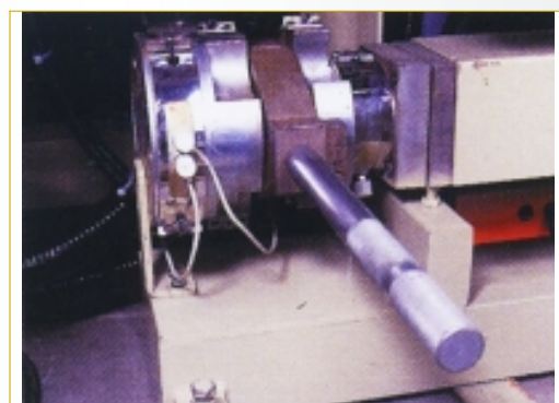
MANUAL SCREEN CHANGER
