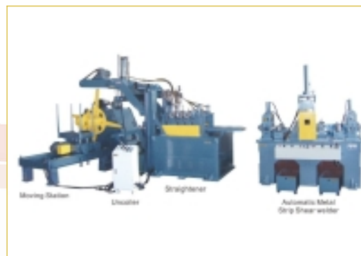
Metallic strip auto shear welder / Automatic Metal Strip Shear welder
