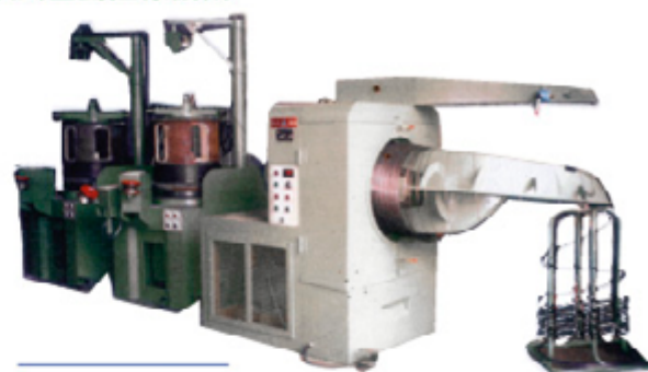
Wire Wiring Machine, Non-Stop Coiler 無段式自動收線機械
