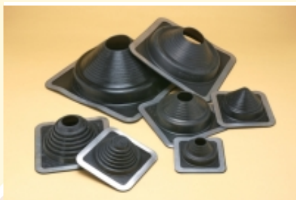
Pipe Flashings
