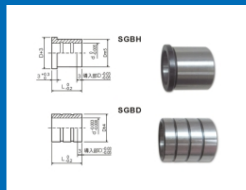
Guide Bush
