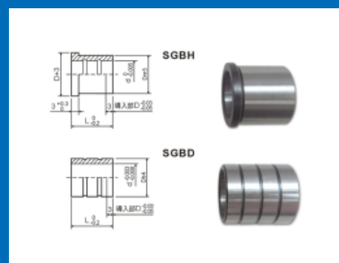
Guide Bush
