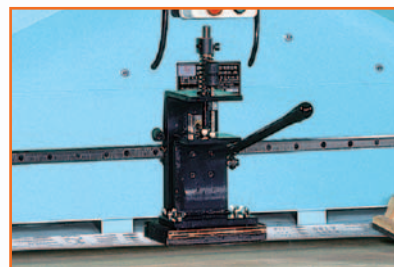
L : Linear motion guide pressure plate 線性滑軌押板
