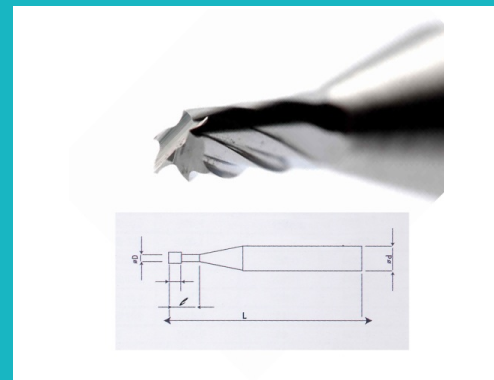
Multiple-flute end Mills
