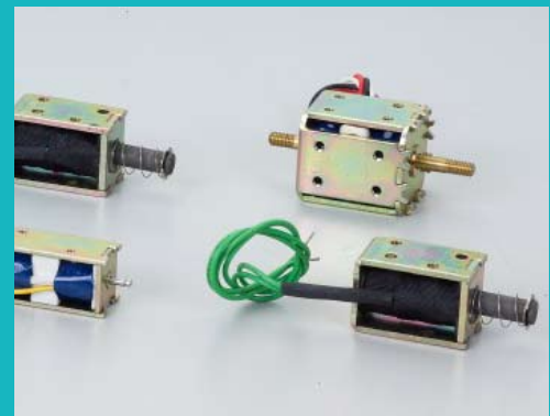
Open Frame Solenoid
