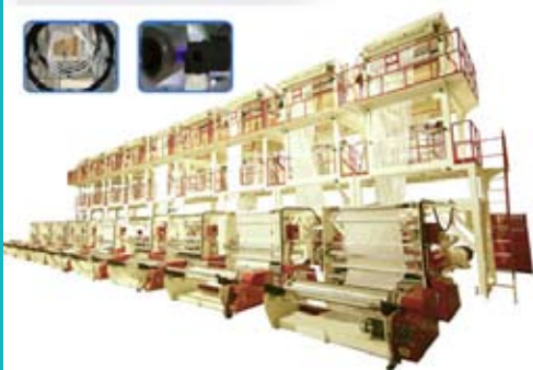
HD/LDPE High Speed Blown Film Machine
