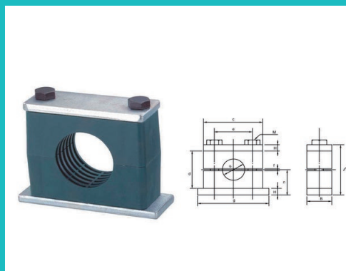
PP High-Pressure Pipe Clamp
