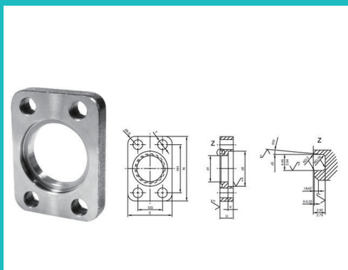
Piping Flange
