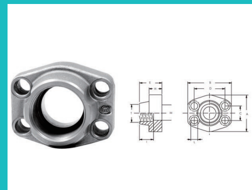
BSP Threaded Flanges
