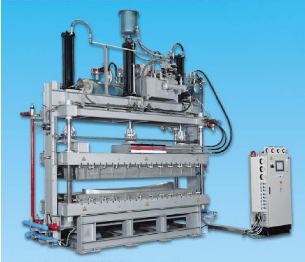
Automatic Vertical EPS / EPE Special-purpose Molding Machine
