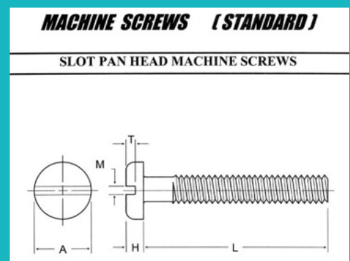
MACHINE SCREWS (STANDARD)
