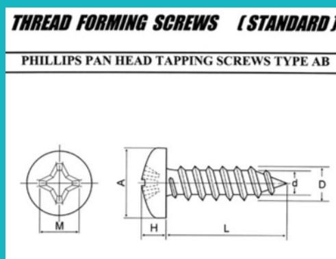
THREAD FORMING SCREWS (STANDARD)
