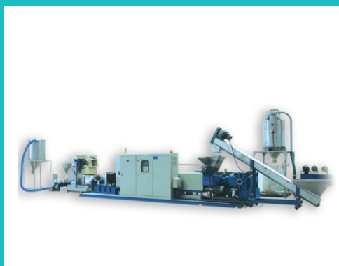
PP/PE Film / Bag / Raffia Extrusion-pelletizing Line (Extruder) by Die Face Cutting
