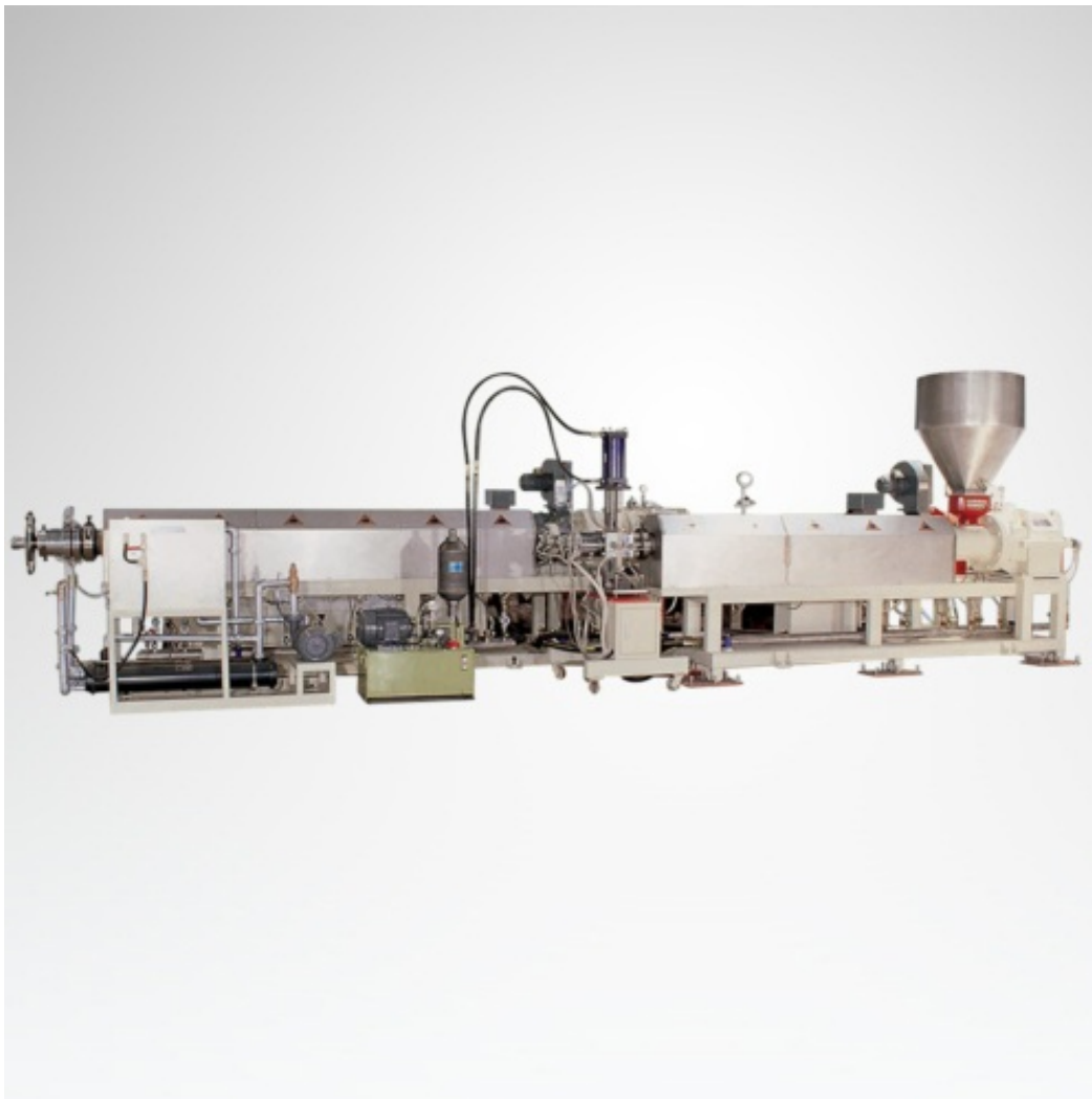
PS/PE Whole Plant Equipment for Manufacturing PS/PE Foamed Sheet
