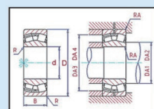
Spherical Roller
