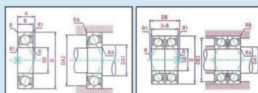
Angular Contact Ball
