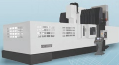
DCM / DCMS Series Double Column Machining Center X Axis: 1700~36000mm Y Axis: 1400~5400mm
