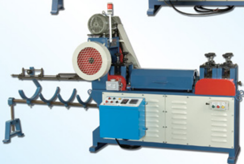
FW-102 Wire Straightening & Cutting Machine
