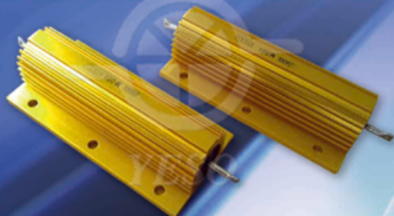
電力型高壓電阻器 High Voltage Glaze Coated Resistors
