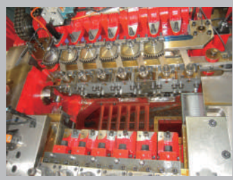
EXTRA FINGER TRANSFER 產品防碰撞機構
