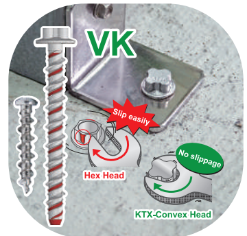
KTX-Concrete Screw
