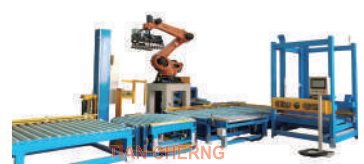
Robot Stack and Wrapping System
