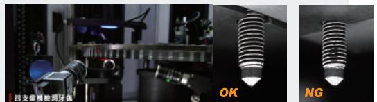
Thread damage checking with 4 cameras
